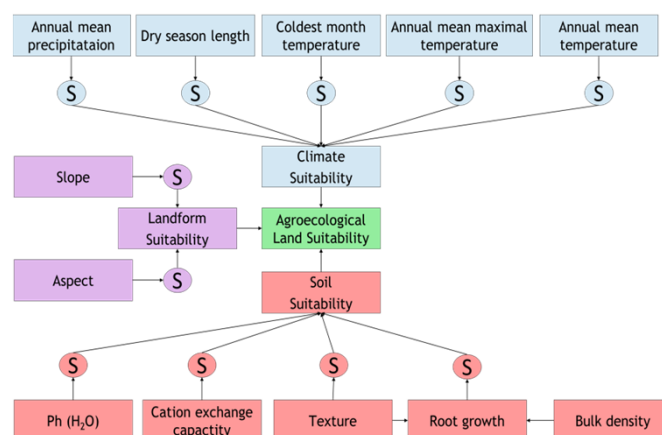
Fig 1. Graphical model of ALECA.
